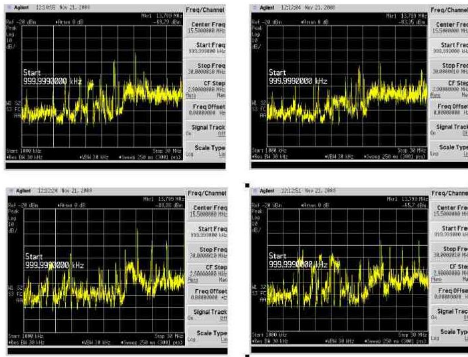
Figure 30 Example of Erratic Noise and Interference
